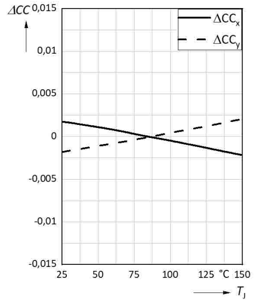
Chromaticity Shift vs. Junction Temperature
