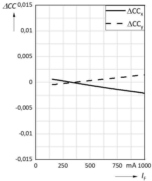
Chromaticity Shift vs. Forward Current
