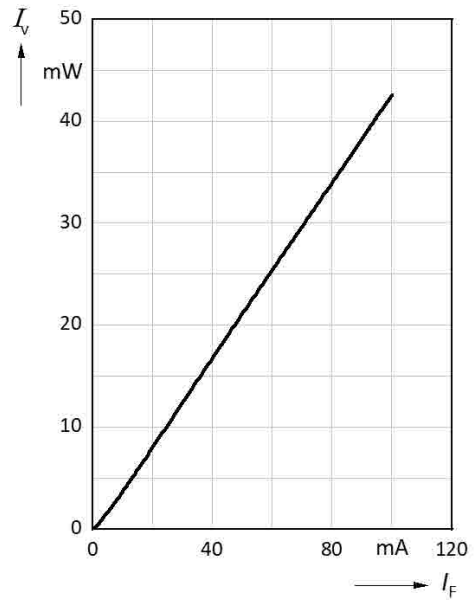
Luminous Intensity vs. Forward Current
