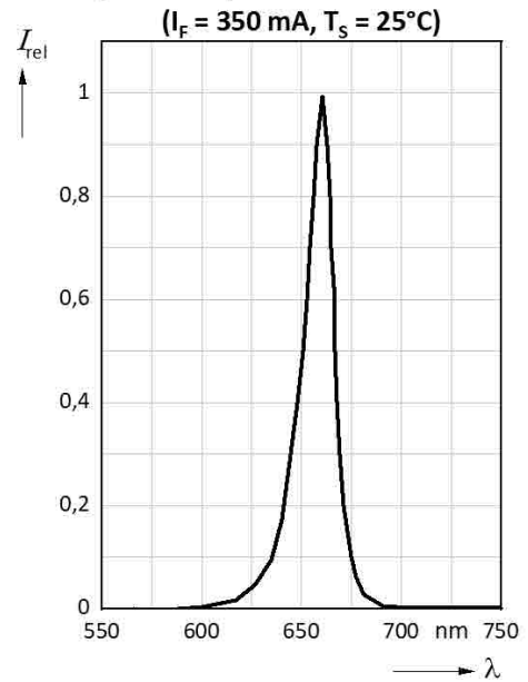
Spektrum (Relative Spectral Emission vs. Wavelength)
