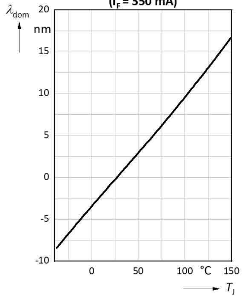
Dominant Wavelength vs. Junction Temperature ( I_F = 350 \text{ mA} )
