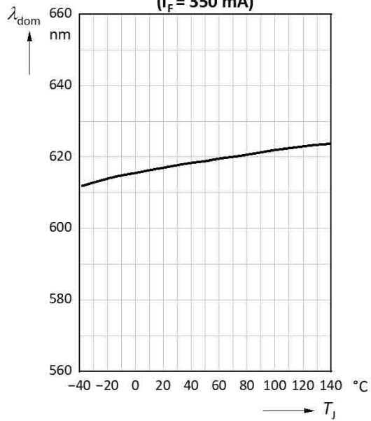
Dominant Wavelength vs. Junction Temperature ( I_F = 350 \text{ mA} )
