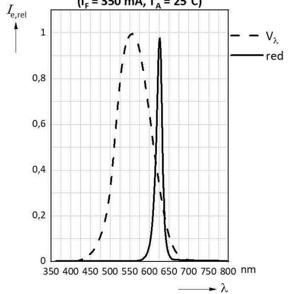
Spectrum (Relative Intensity vs. Wavelength) ( I_F = 350 \text{ mA} , T_A = 25^{\circ}\text{C} )
