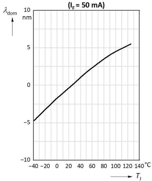
Dominant Wavelength vs. Junction Temperature
