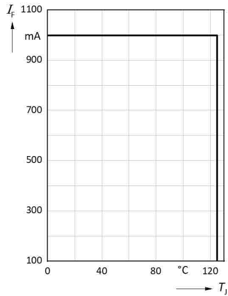
Forward Current vs. Junction Temperature
