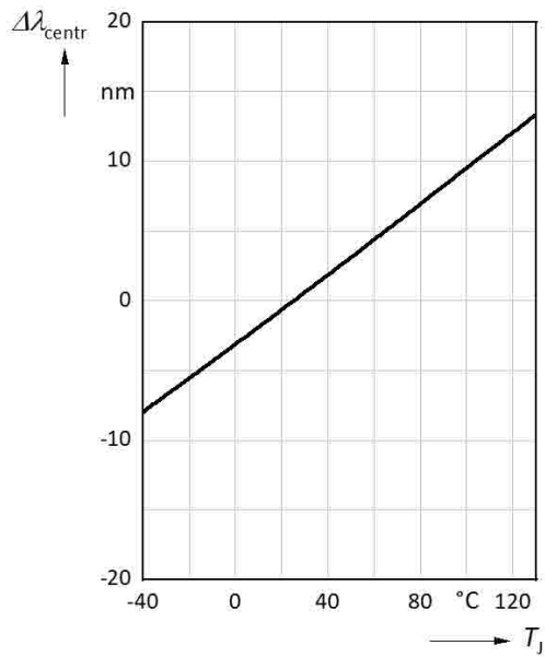
Centroid Wavelength Shift vs. Junction Temperature
